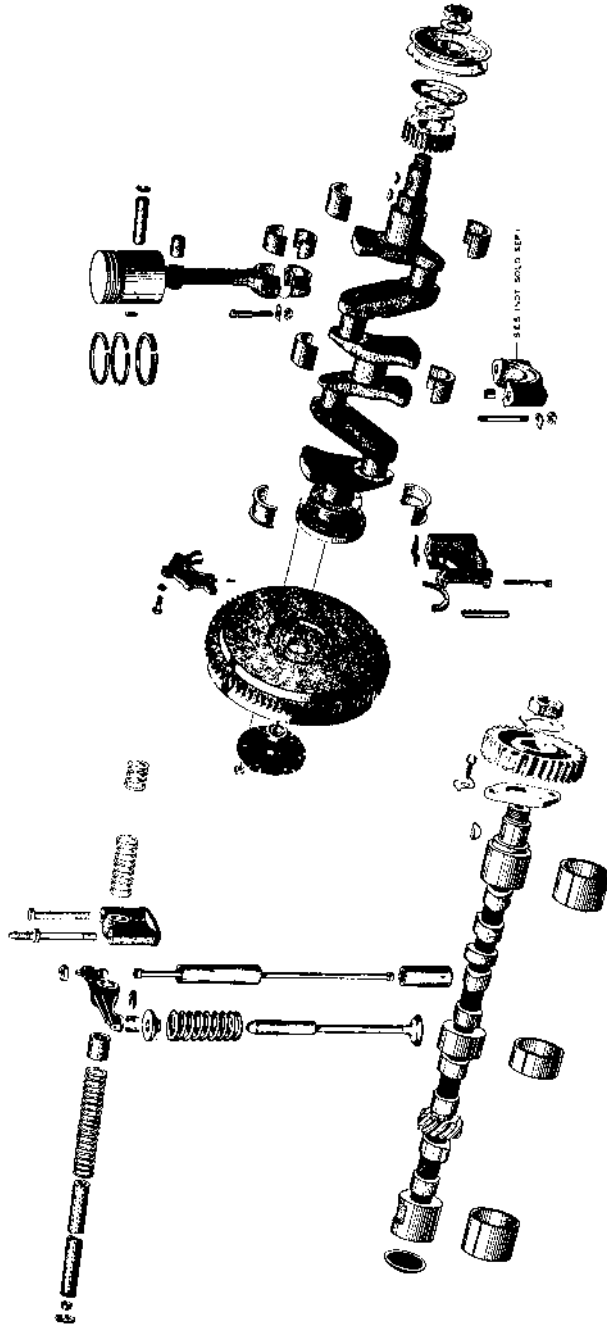
Ventilmekanism.
