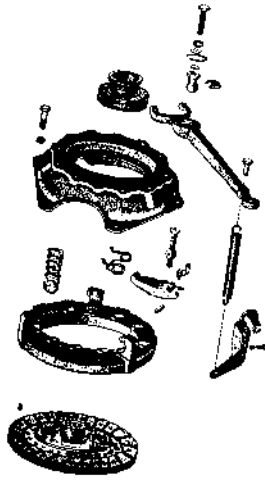
Koppling.
